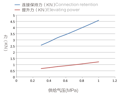
OQX-30 continuous relay and lifting force curve
