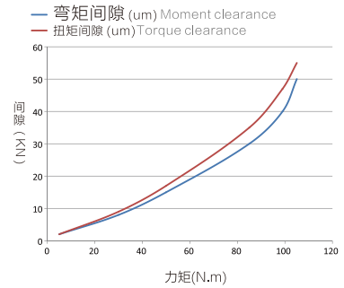
OQX-30 Bending moment and torque changer curve
